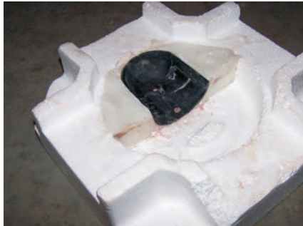
The existing cap was used to make a female mold in the thickened epoxy.
